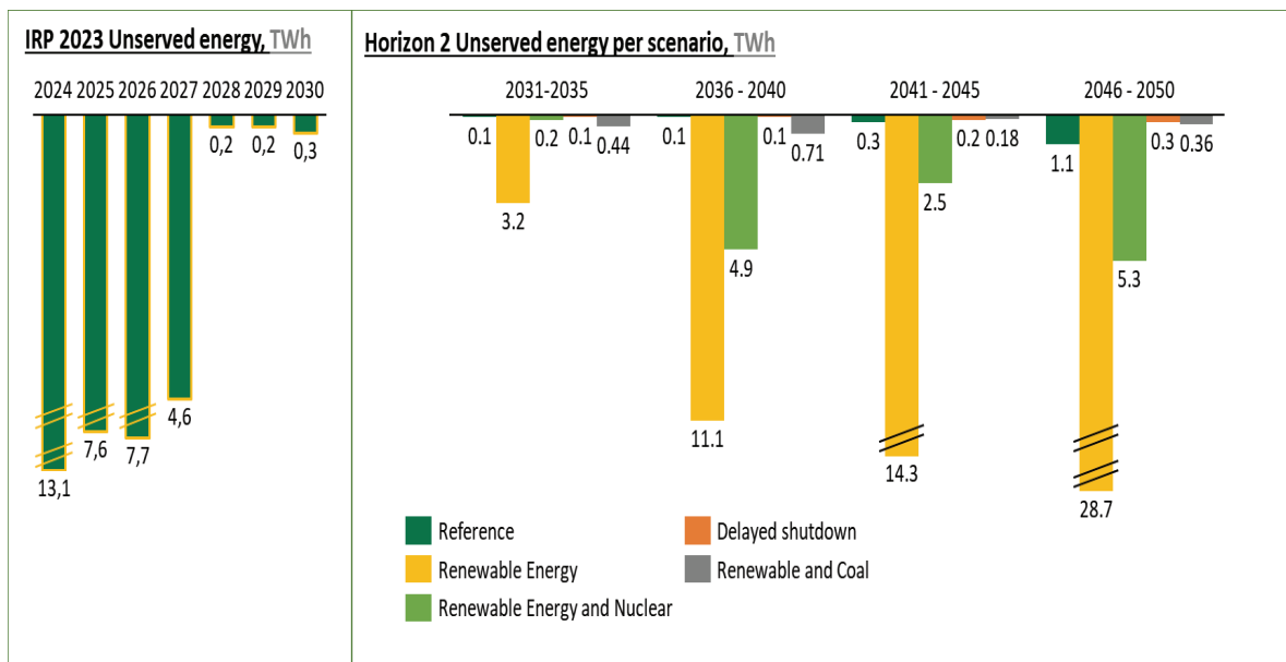
Figure 20: Unserviced Energy as an indicator of security of supply
