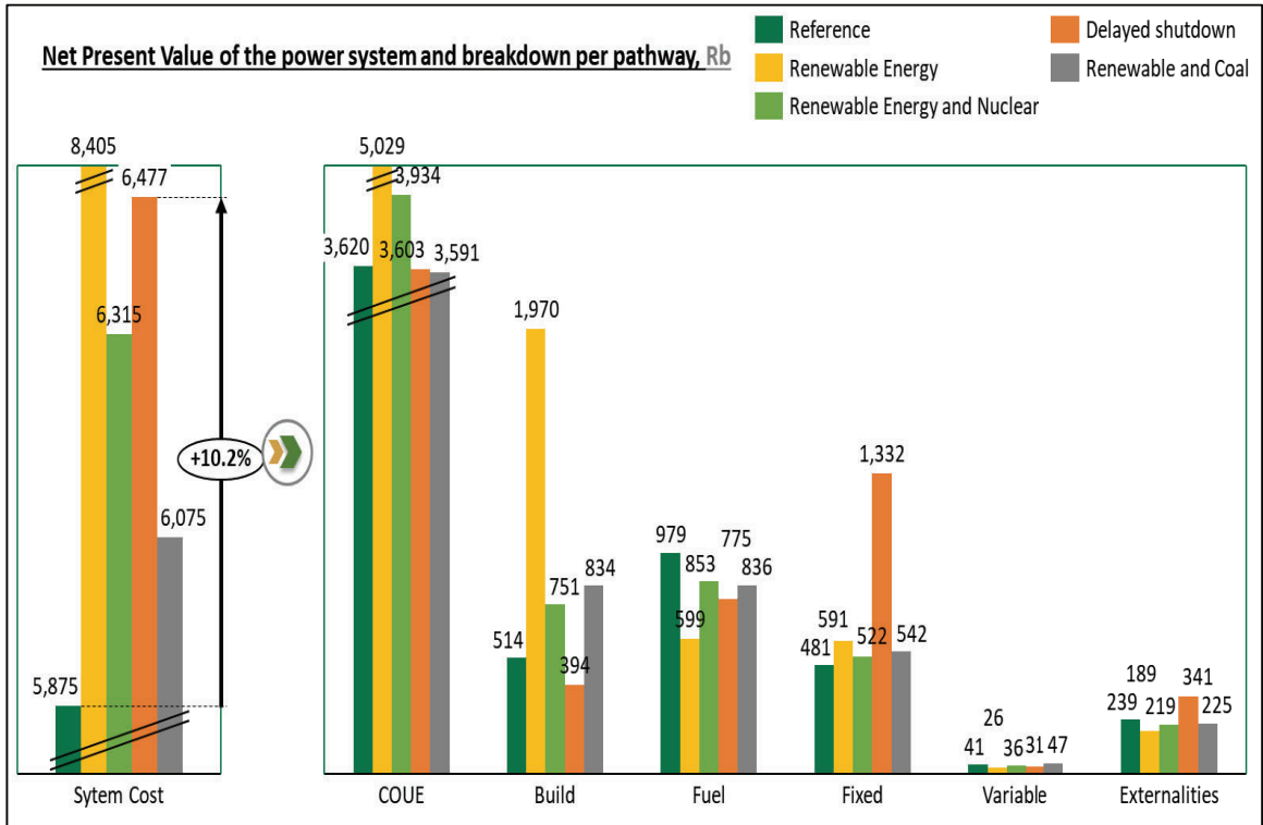
Figure 22: Power system costs associated with the pathways studied
